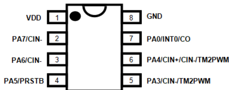
PMS15B/PMS150G-S08: SOP8 (150mil)
