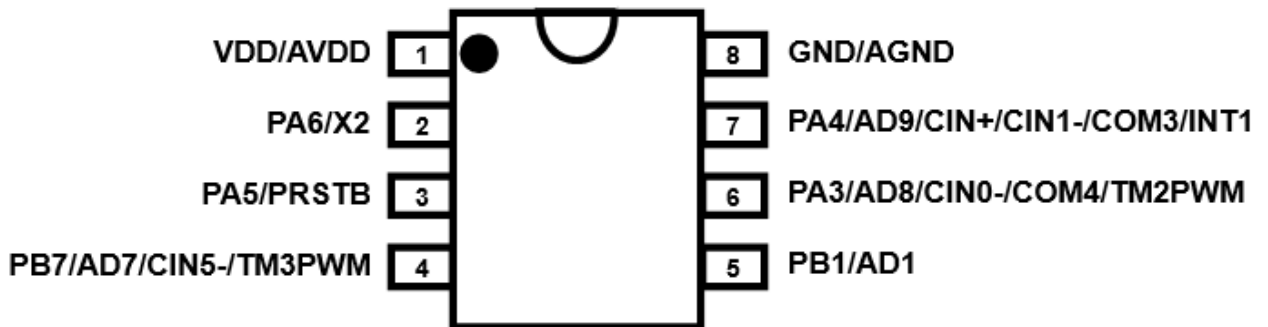
PFS122B-S08 (SOP8-150mil)
