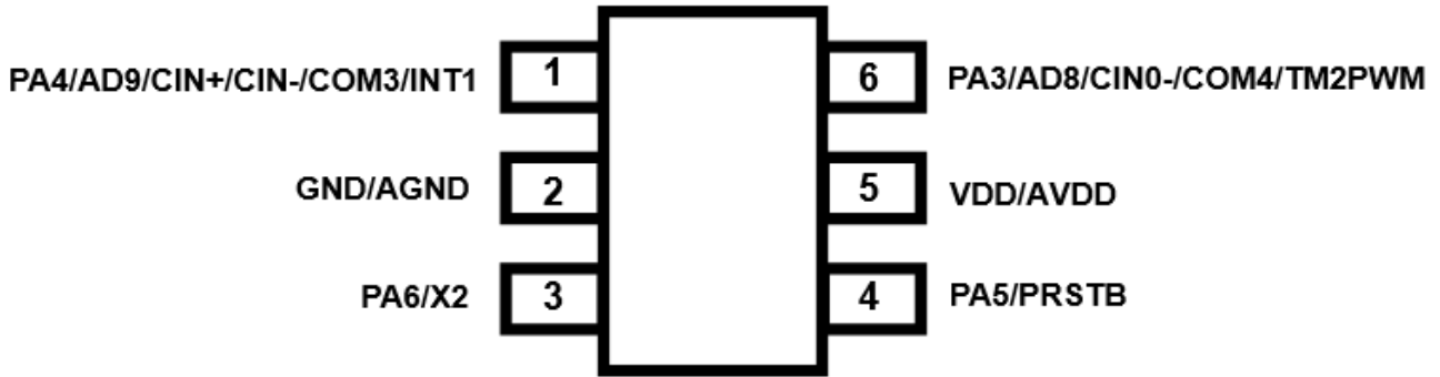
PFS122B-U06 (SOT23-6 60mil)
