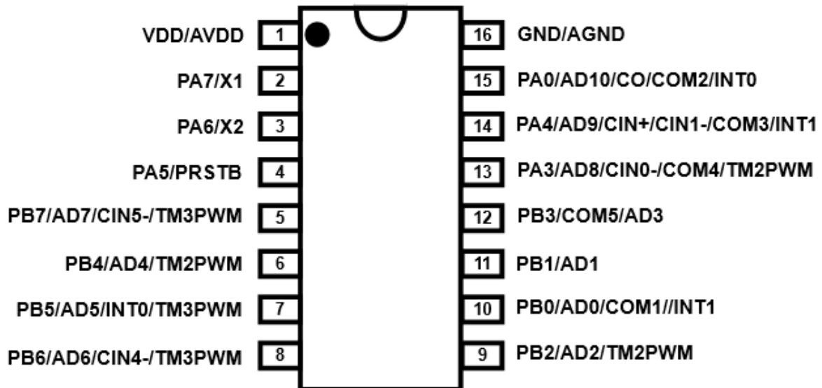
PFS122B-S16A (SOP16A-150mil)
