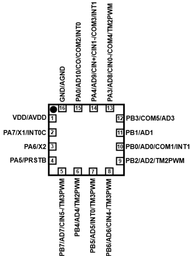
PFS122B-1J16A (QFN3*3-16pin-0.5pitch)
