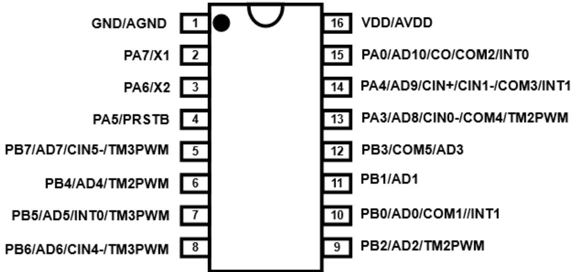
PFS122B-S16B (SOP16B-150mil)
