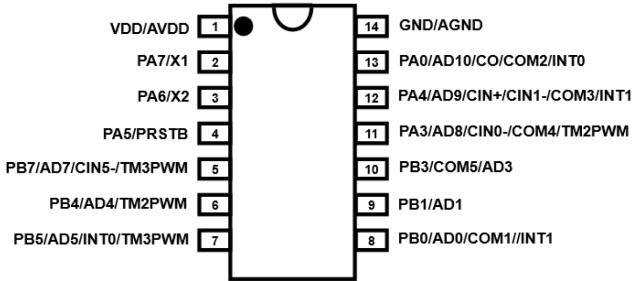
PFS122B-S14 (SOP14-150mil)
