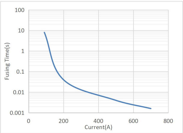
Various interrupting current at 25℃ ambient temperature Constant
