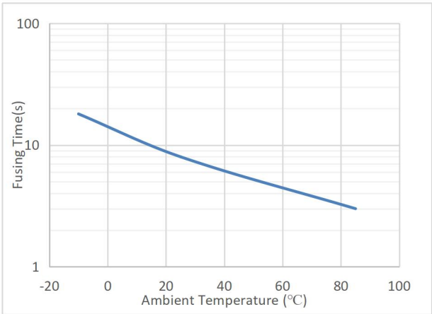
2x rated current at various ambient temperature
