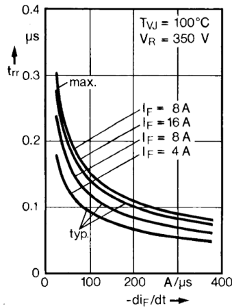
Fig. 5 Recovery time versus -di_F/dt .
