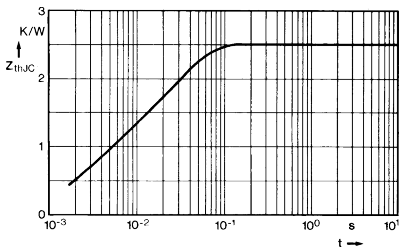
Fig. 7 Transient thermal impedance junction to case.
