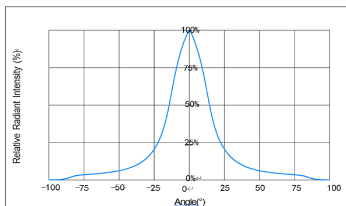
Fig 6 Diagram characteristics of radiation 辐射特性曲线
