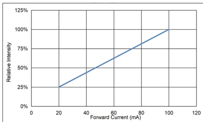
Fig 2 Forward Current Vs Relative Intensity 正向电流与相对光强特性曲线
