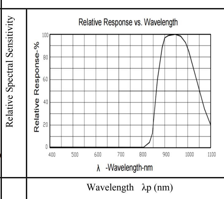
Fig.2 Spectral Distribution
