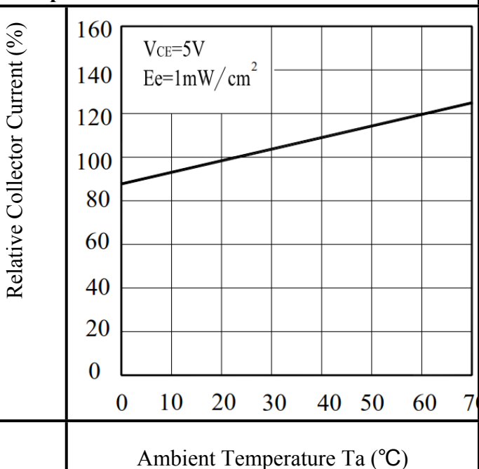
Fig.3 Relative Collector Current vs. Ambient Temperature
