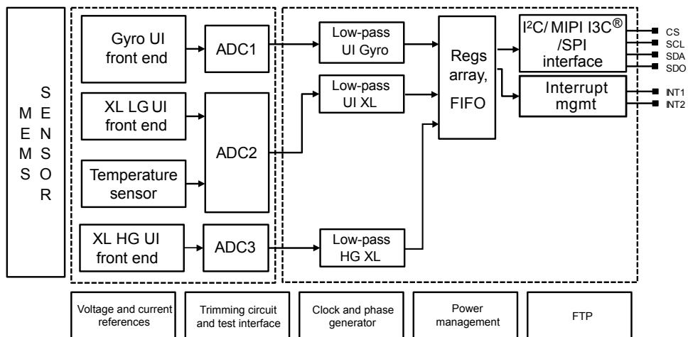
Figure 18. Block diagram of filters
