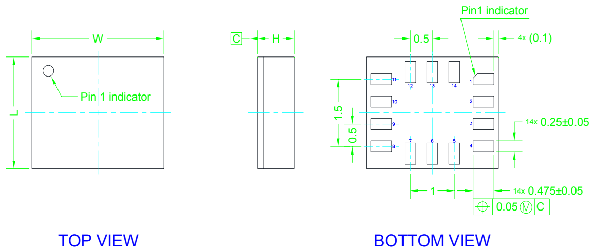
Figure 25. LGA-14L 2.5 x 3.0 x 0.83 mm package outline and mechanical data
