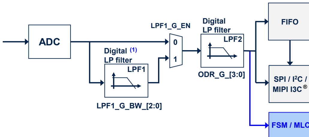
Figure 21. Gyroscope digital chain
