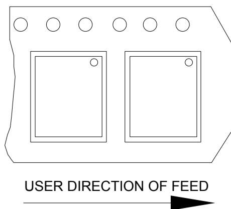
Figure 27. LGA-14L package orientation in carrier tape
