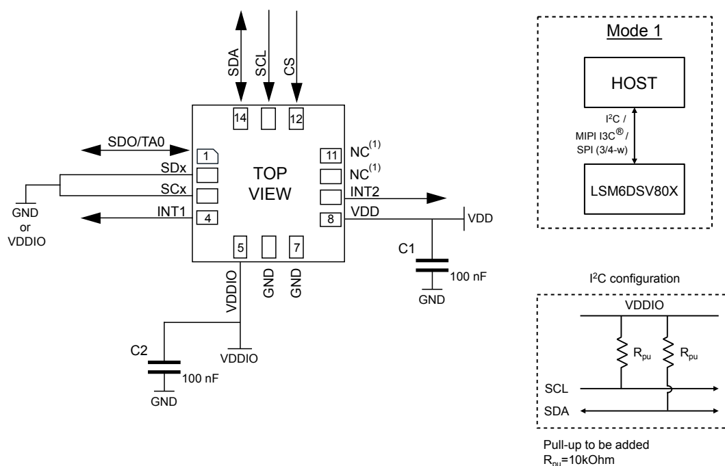
Figure 22. LSM6DSV80X electrical connections in mode 1
