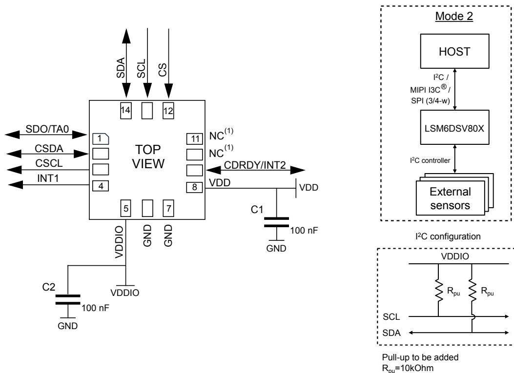
Figure 23. LSM6DSV80X electrical connections in mode 2
