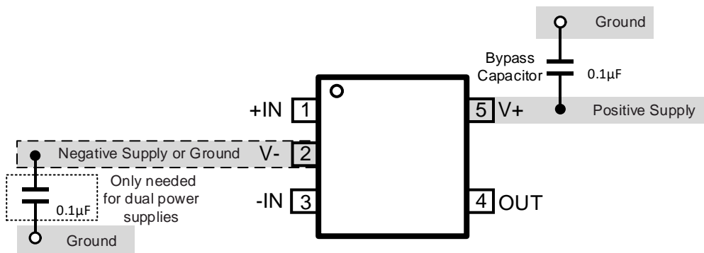
Figure 4. TL331IDBVR-MS Layout Example
