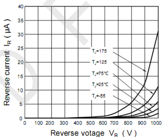
Figure 2. Reverse Characteristics
