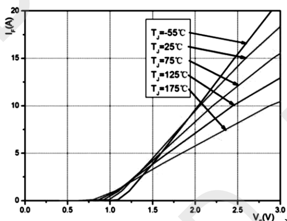
Figure 1. Forward Characteristics
