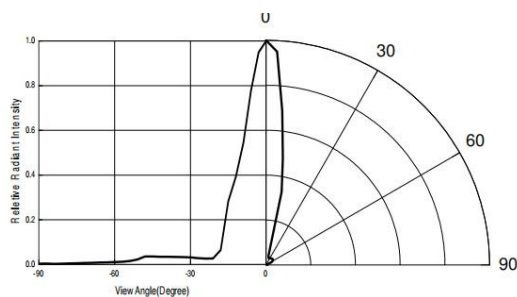
Fig. 7 Relative Radiant Intensity vs. Angular Displacement
