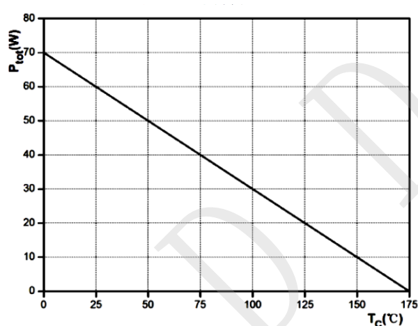
Figure 4. Dissipated power curve
