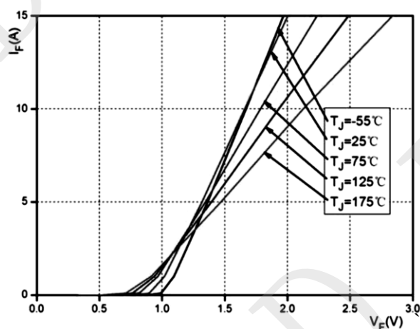
Figure 1. Forward Characteristics
