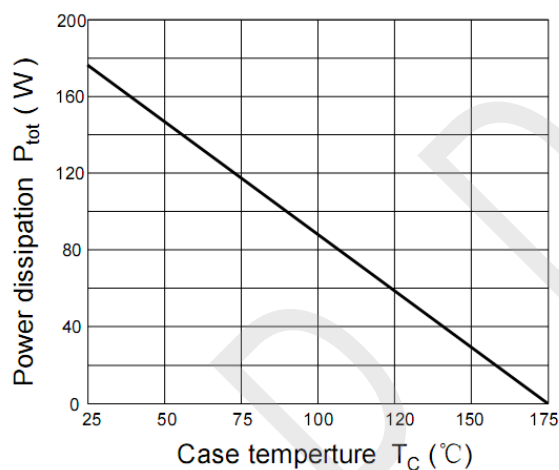
Figure 4. Power Derating
