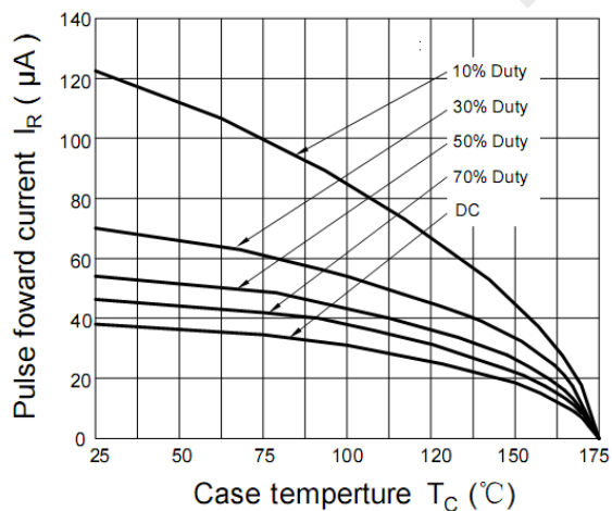
Figure 3. Current Derating
