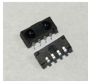
1, 4 = GND, 2 = VS, 3 = OUT
