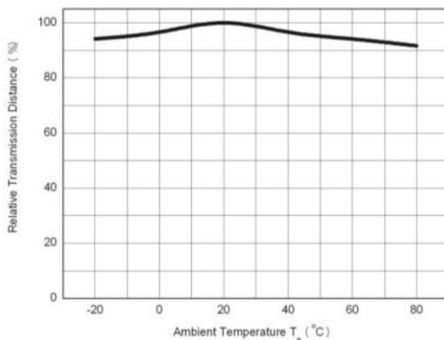
4、Relativi Transmission Distance VS. Ambient Temperature
