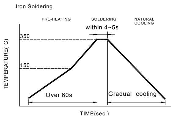
Fig.2 Iron soldering temperature profiles
