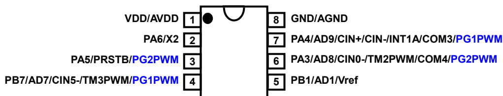
PFS132-S08 (SOP8-150mil)
