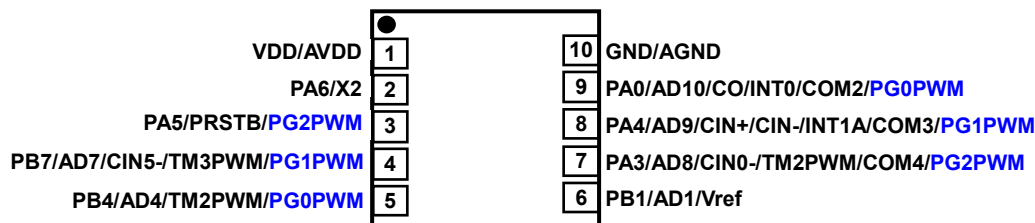
PFS132-4N10 (DFN3*3-10P-0.5pitch)
