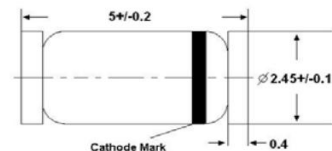
Glass case MELF Dimensions in mm
