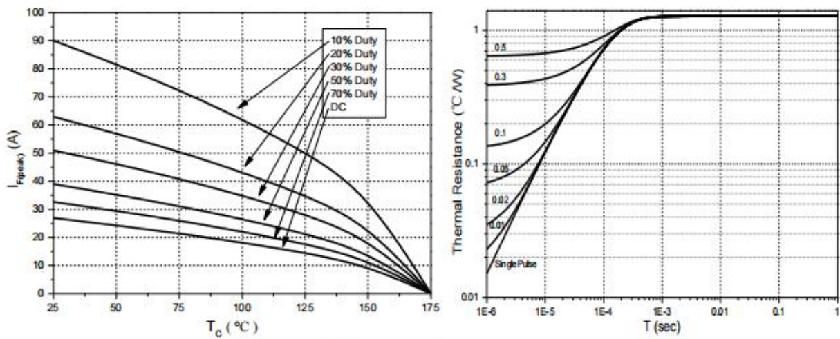
Figure 7. Current Derating Figure 8. Transient Thermal Impedance
