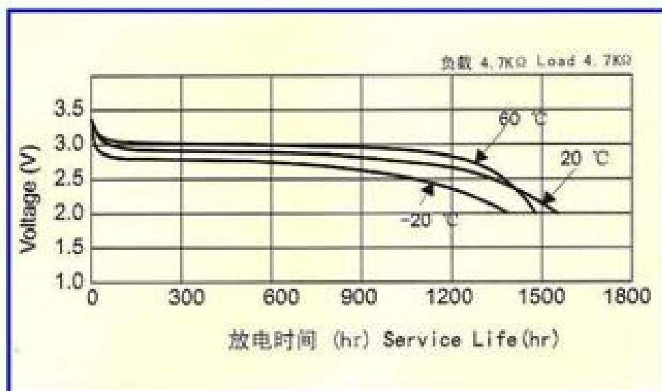
Temperature Characteristics
