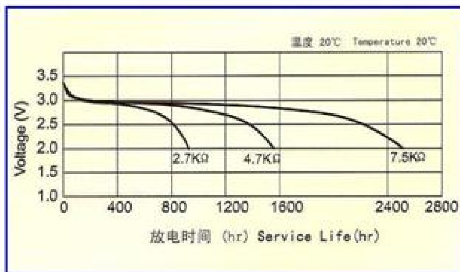
Discharge Characteristics
