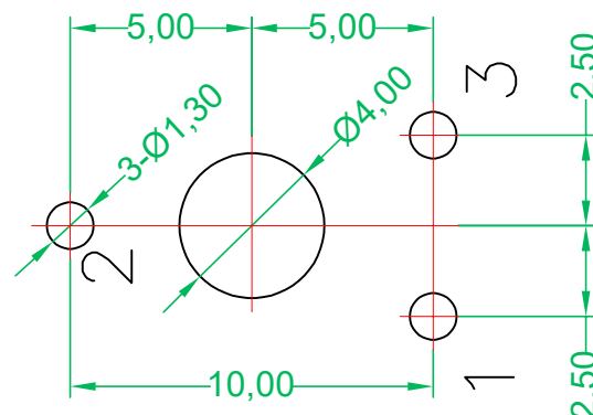
PC板固定孔圖 P.C.B. MOUNTING HOLE DETAIL
