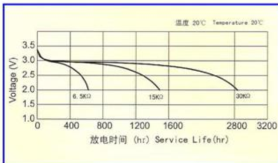
Discharge Characteristics
