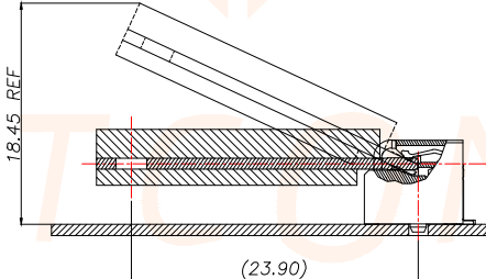
EJECT HEIGHT FOR HALF CARD
