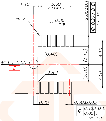
DETAIL D SCALE 2:1
