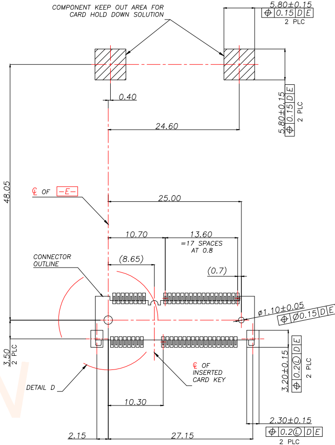
-D- IS THE TOP SURFACE OF PCB. RECOMMENDED P.C. BOARD PATTERN LAYOUT FOR FULL CARD CONNECTOR (TOP VIEW)
