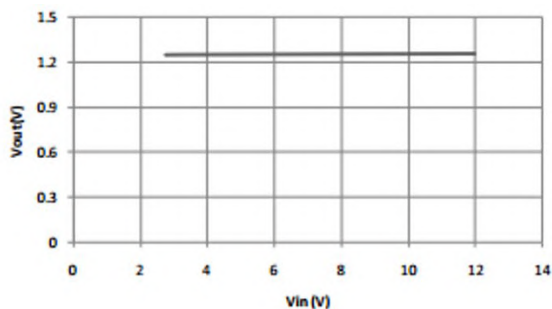
Line regulation ICW1117-ADJ V_{out} Vs. V_{in}
