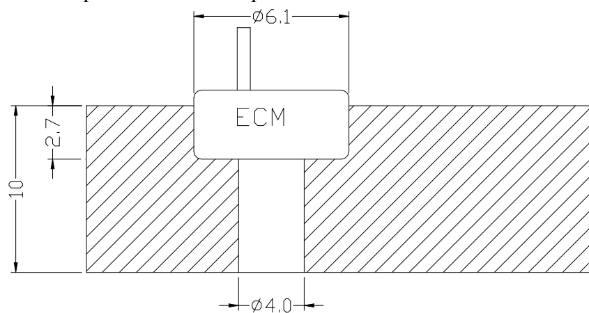
7-8 固定部孔形状 Shape of hole at fixed part
