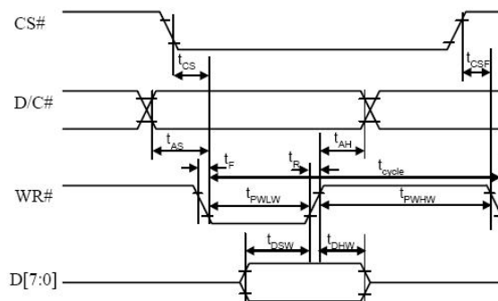
( Write Timing )
