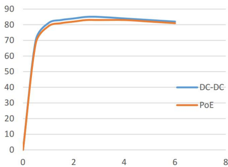
效率(Vout = 5V)
