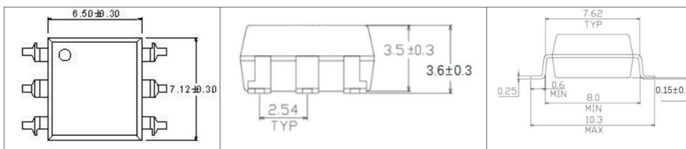
6-pin SMD
