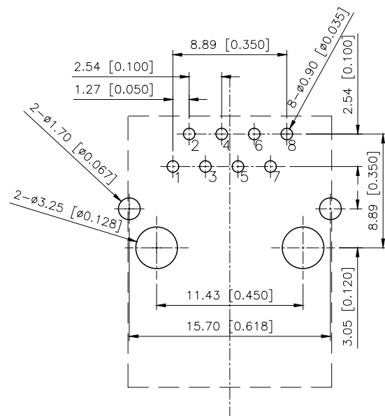
RECOMMENDED PCB LAYOUT VIEWED FROM COMPONENT SIDE
