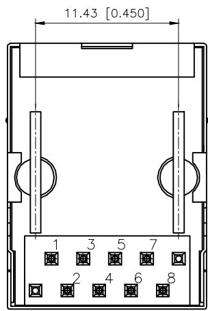
BOTTOM VIEW
