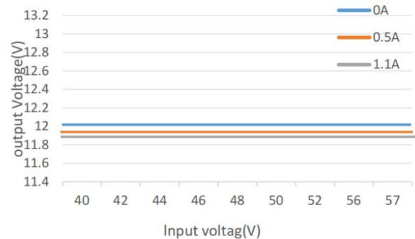
Input voltage & output voltage
