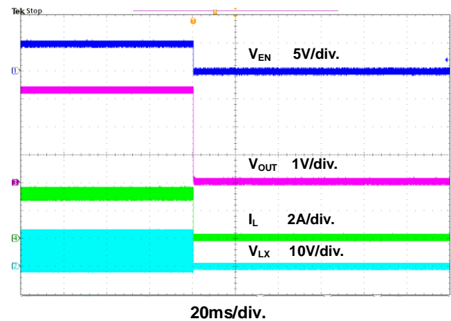
Figure 10. Power Off through \overline{SHDN} Waveform
