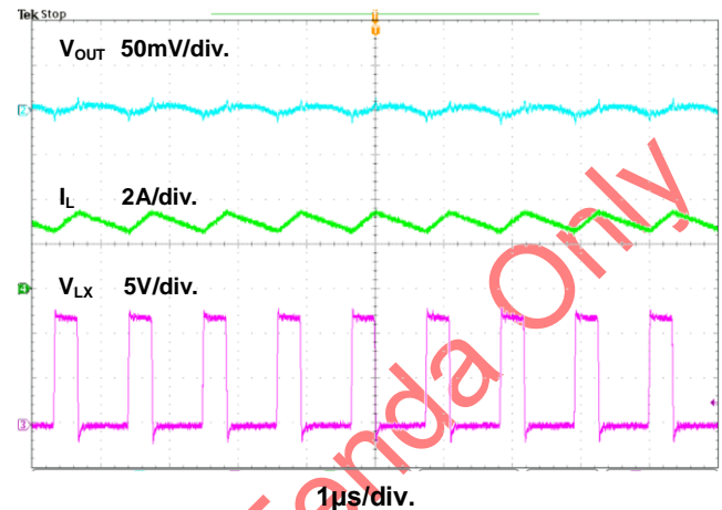
Figure 6. Steady State Waveform
