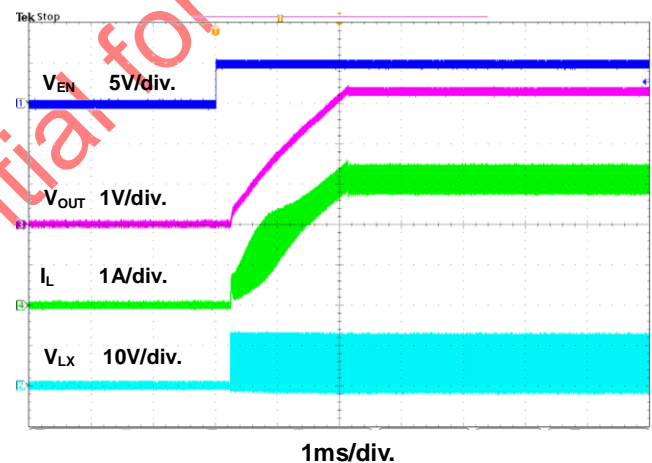
Figure 8. Power On through \overline{SHDN} Waveform
