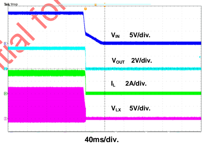
Figure 14. Power Off through VIN Waveform
