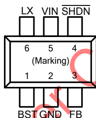
Figure 1. Pin Assignments of FR8205A
