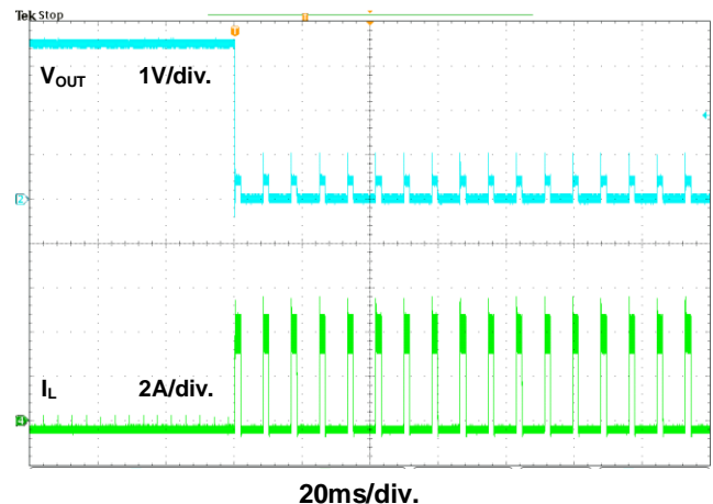
Figure 16. Short Circuit Test
