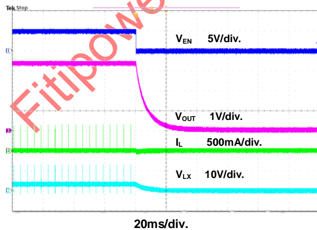
Figure 9. Power Off through \overline{SHDN} Waveform
