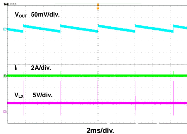
Figure 5. Steady State Waveform
