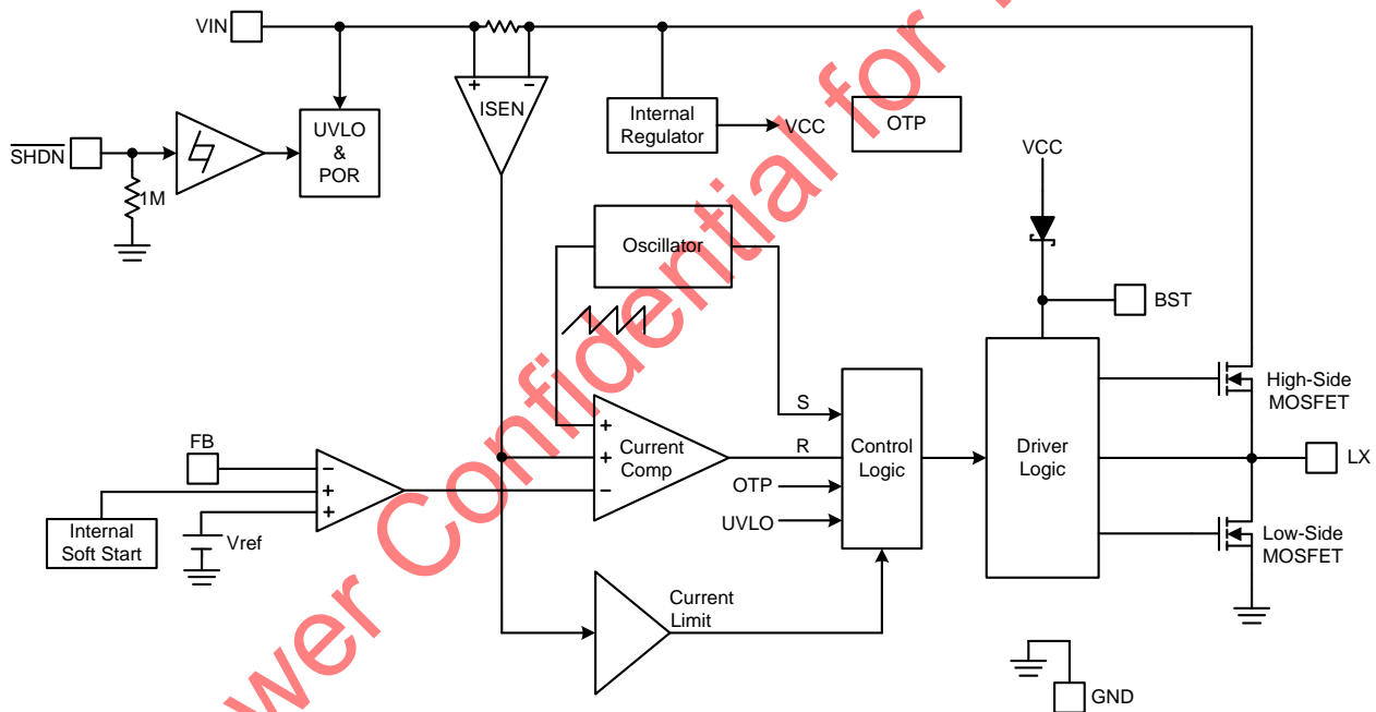
Figure 4. Block Diagram of FR8205A
