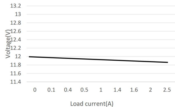
Output current voltage (input 48V)
