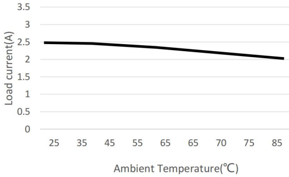
Derating
