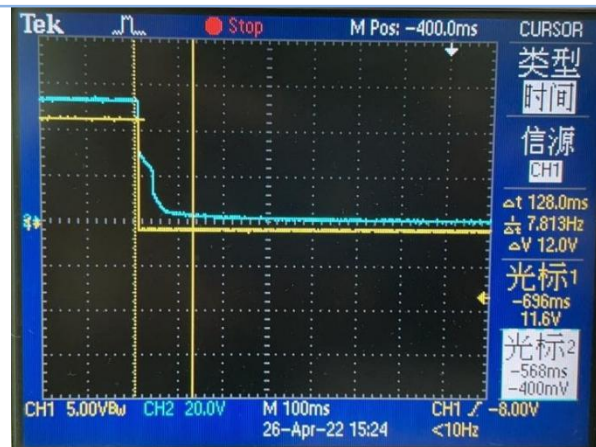
Power Down
