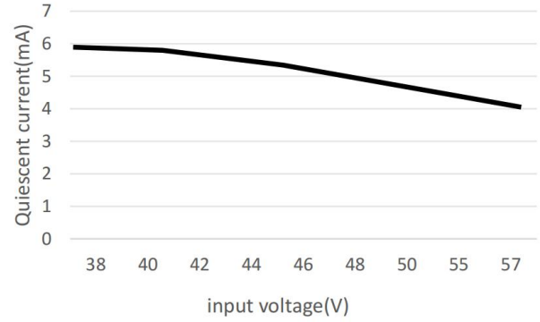
Quiescent current
