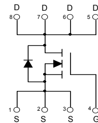
Equivalent Circuit
