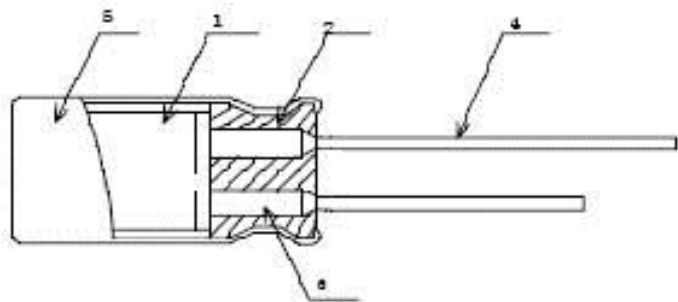
Fig. 1 Cross-section view
