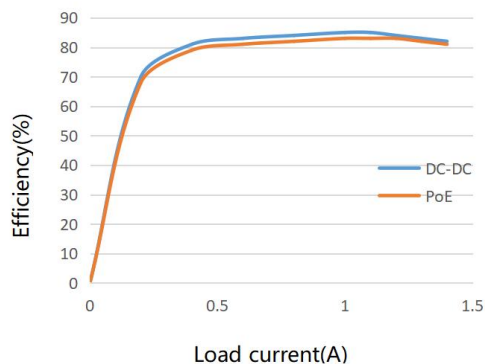
Efficiency (Vout = 12V)
