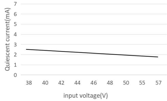
Quiescent current
