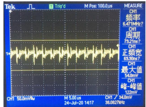
Output ripple (12V/1.1A)
