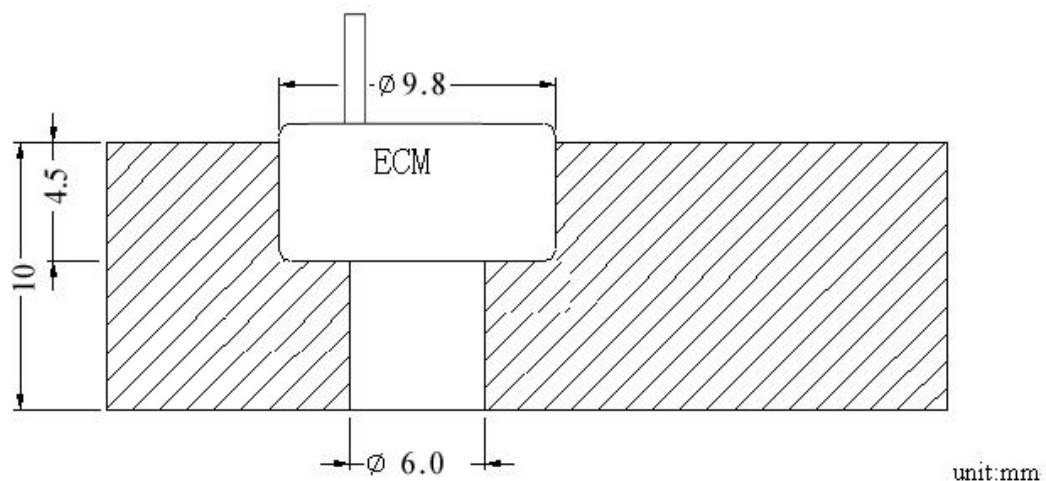
7-8 固定部孔形状 Shape of hole at fixed part
