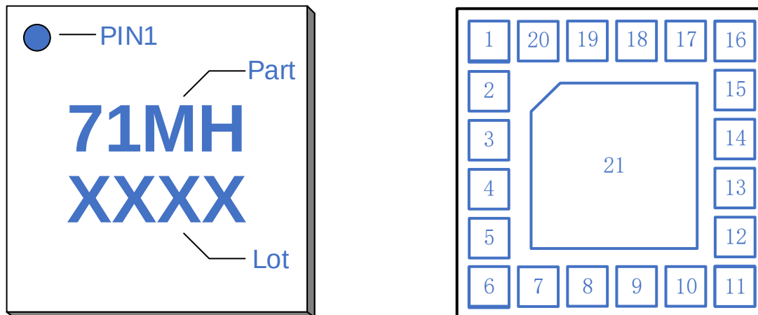
Figure 2 Pin-out Information
