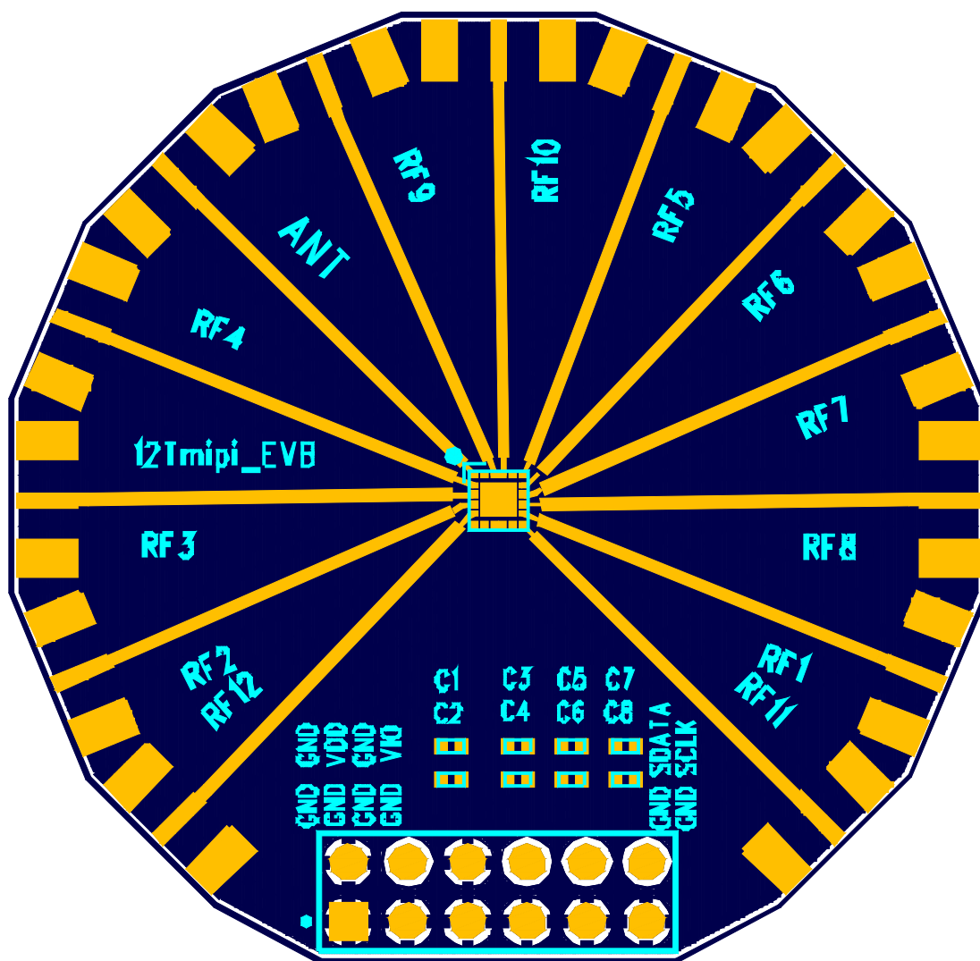
Figure 4 Evaluation Board Assembly Diagram
