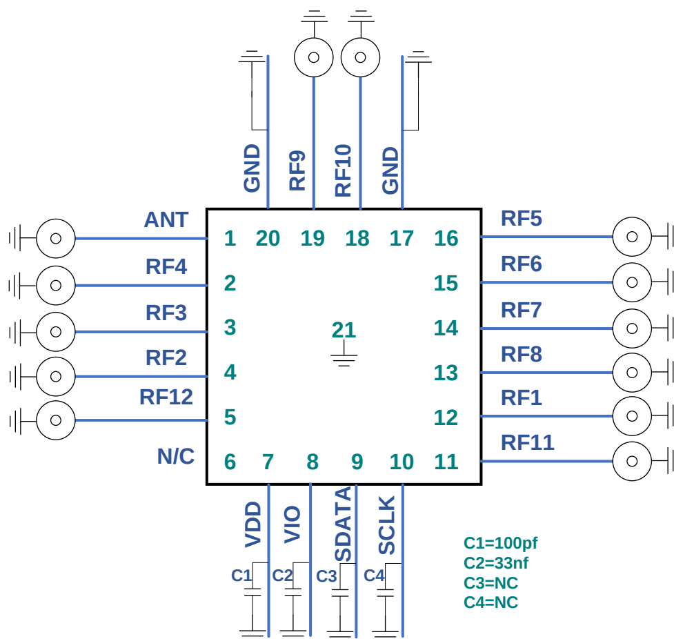
Figure 3 Application circuit
