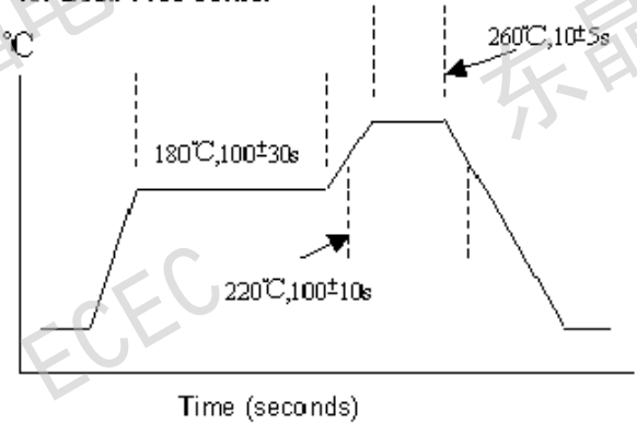
Recommendation of flow condition for Lead-Free solder
