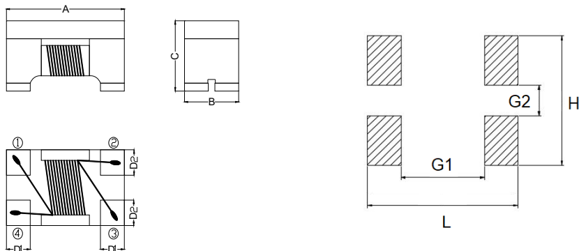
Recommended PC Board Pattern
