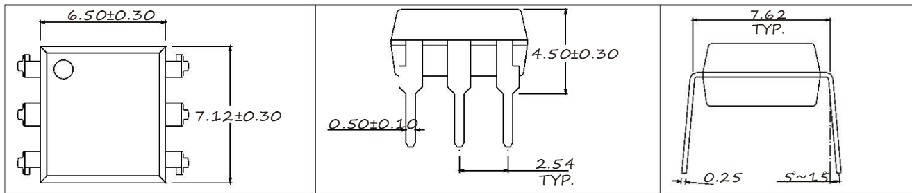
6 pin DIP
