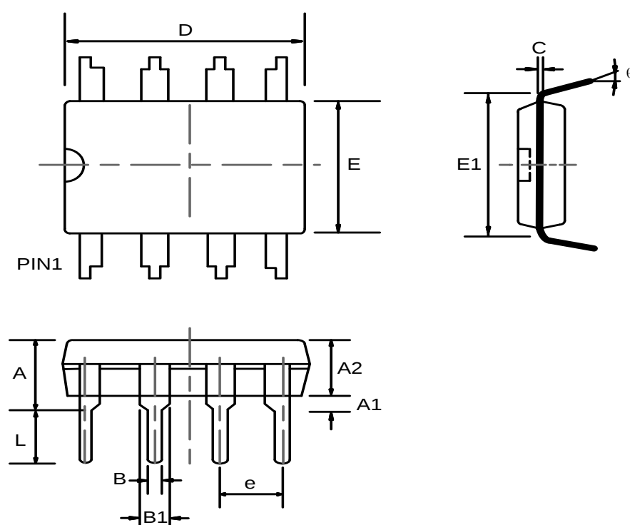
DIP8 package mechanical drawing
