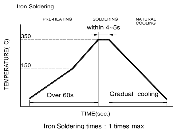
Fig.2 Iron Reflow
