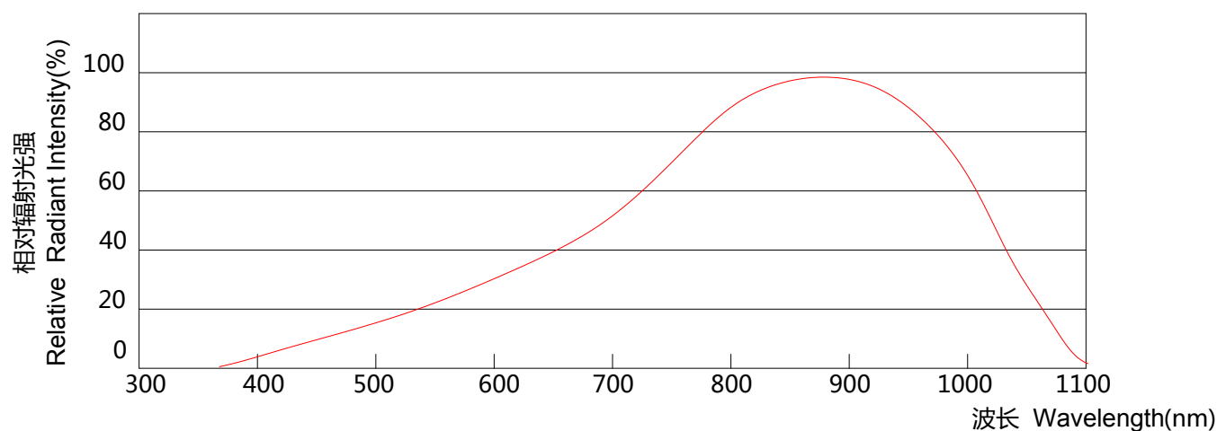
感光特性曲线 Photographic property Curve
