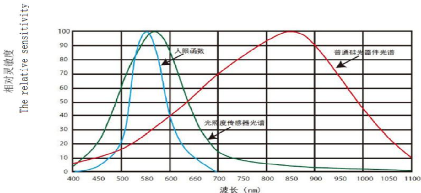
图 1-1 Photoreceptor curve PT850 Visible light sensor curve
