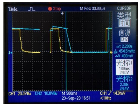
Output response &amp; load (24V / 1.25A)
