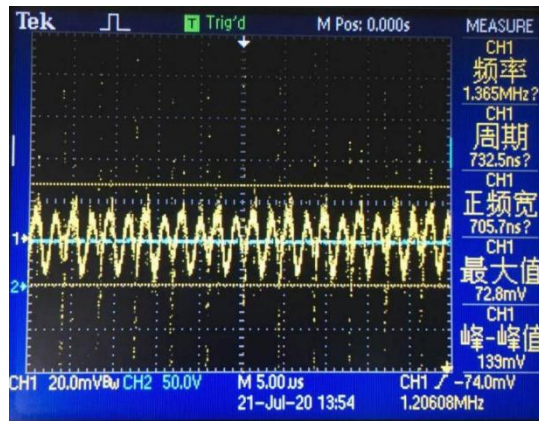
Ripple wave (VIN = 42V, IO = 1.25A, 5 ~ 20MHz bandwidth)
