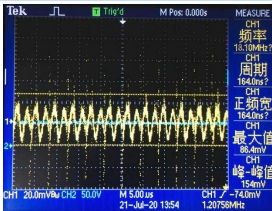
Ripple wave (VIN = 48V, IO = 1.25A, 5 ~ 20MHz bandwidth)
