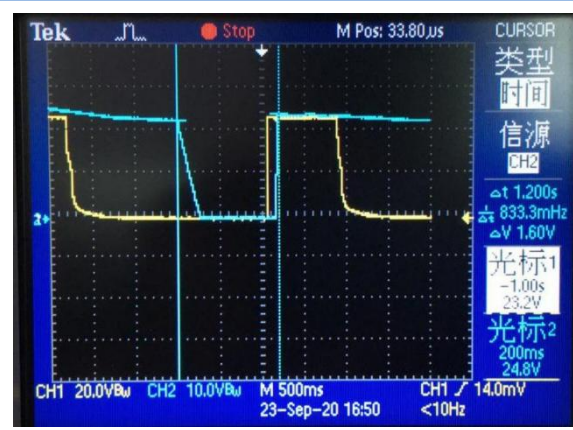
Output response &amp; load (24V / 0.6A)
