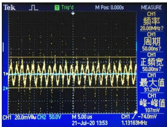
Ripple wave (VIN = 57V, IO = 1.25A, 5 ~ 20MHz bandwidth)
