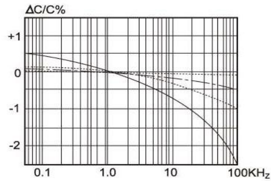
Capacitance vs.Frequency 容量与频率
