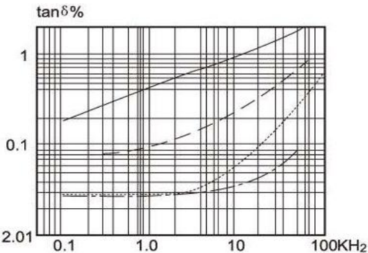
Dissipation factor vs.Frequency 损耗与频率
