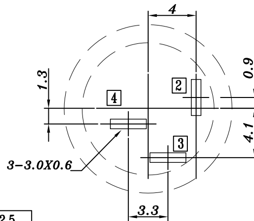
PCB LAYOUT
