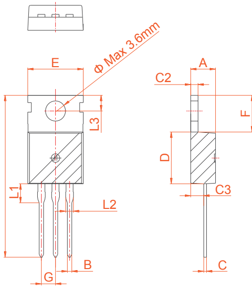
TO-220C
