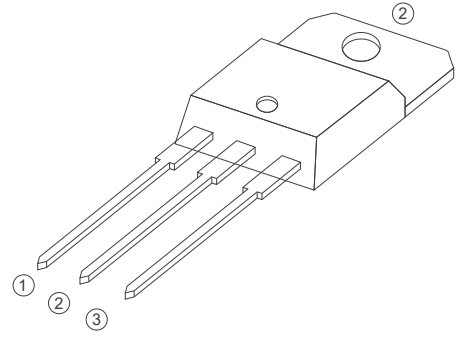
TO-220B Non-Insulated
