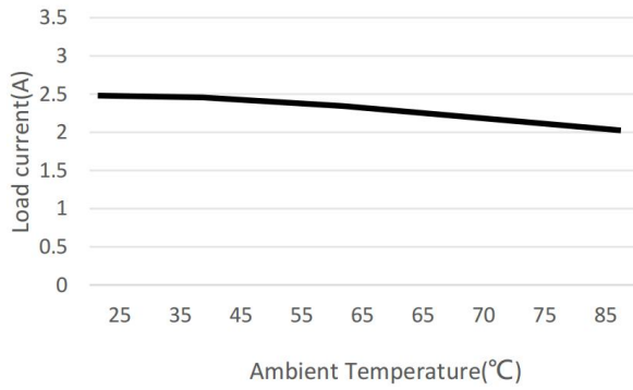
Derating
