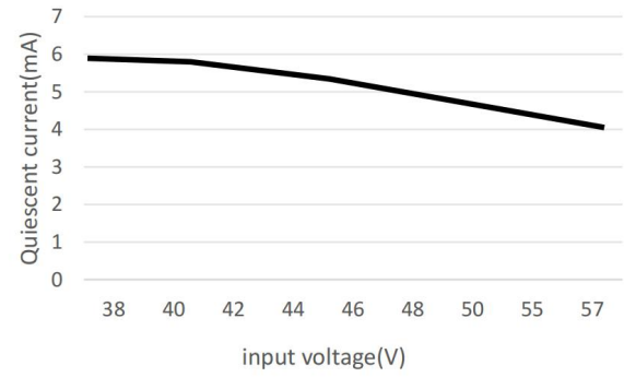
Quiescent current
