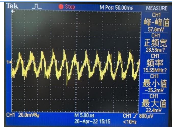
Output ripple (12V / 2.5A)
