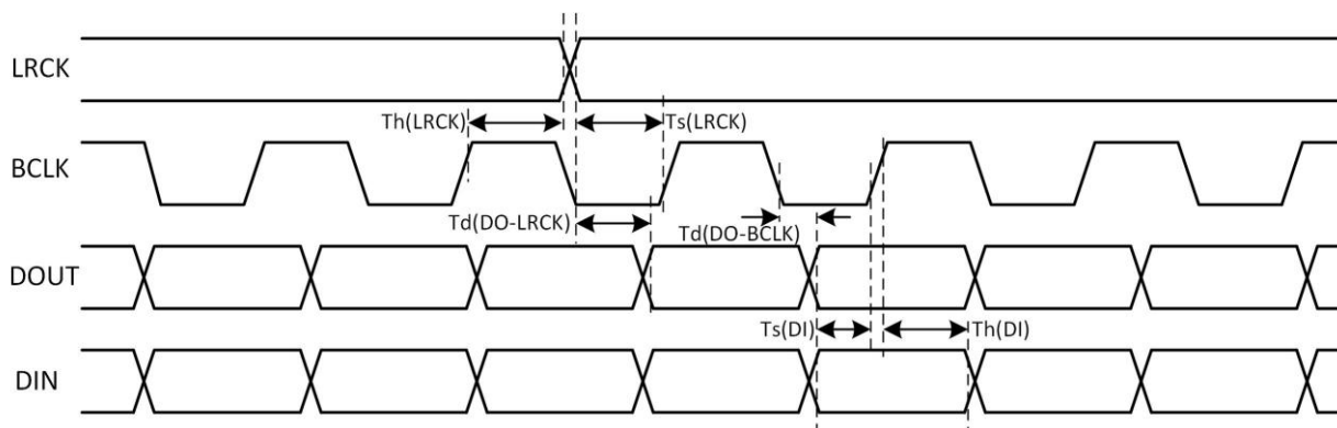
Figure 5-39. I2S/PCM Timing in Slave Mode
