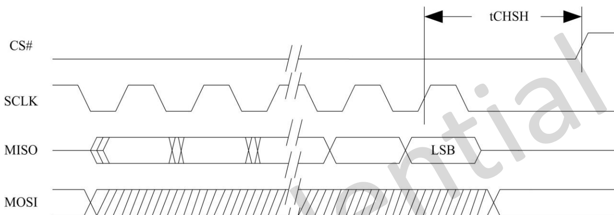
Figure 5-32. SPI MISO Timing
