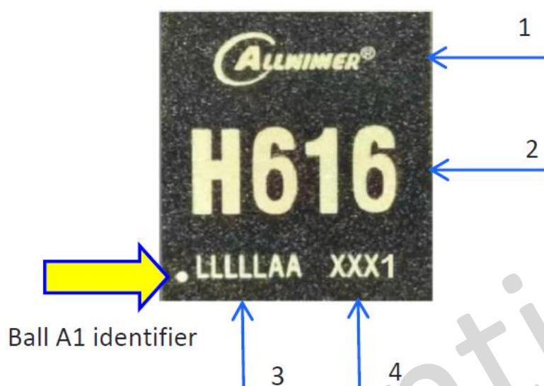
Figure 11-1. H616 Marking
