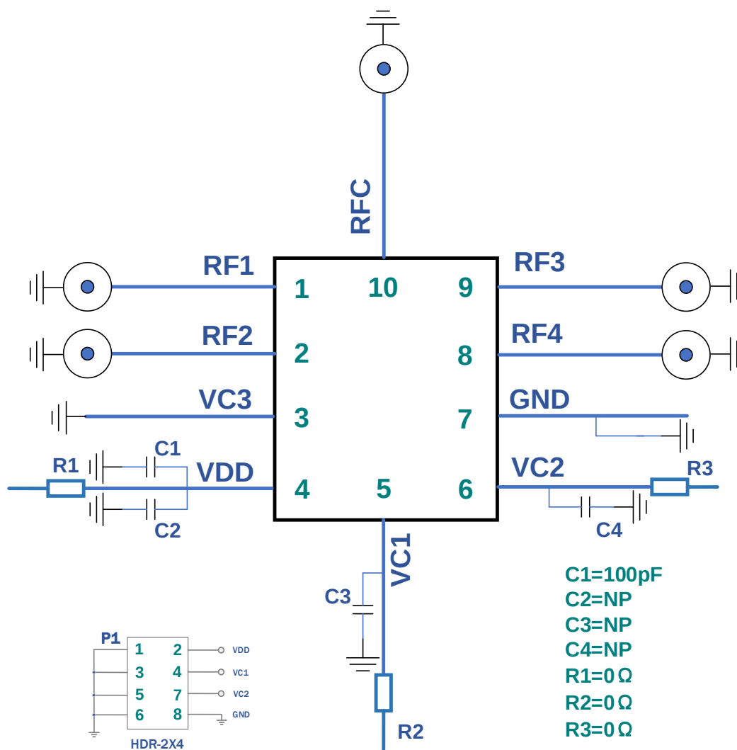
Figure 3 Application circuit
