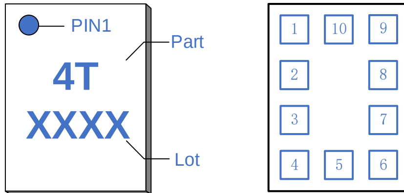
Figure 2 Pin-out Information
